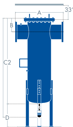
Flanged Filters
